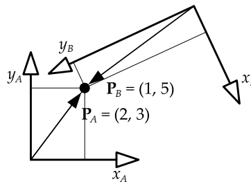
Figure 4.17. Position vectors for the point P relative to different coordinate axes.
