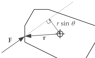
Figure 12.25. Torque is calculated by taking the cross product between a force's point of application in body space (i.e., relative to the center of mass) and the force vector. The vectors are shown here in two dimensions for ease of illustration; if it could be drawn, the torque vector would be directed into the page.
