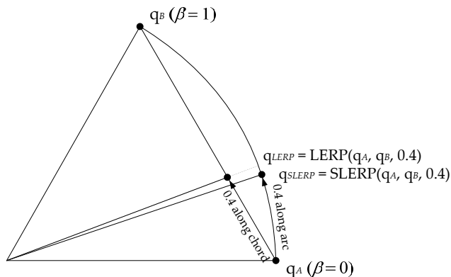
Figure 4.24. Spherical linear interpolation along a great circle arc of a 4D hypersphere.
