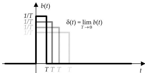
Figure 13.12. The unit impulse can be defined as the limit of a box function b(t) whose width approaches zero.
