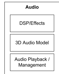
Figure 1.31. Audio subsystem.
