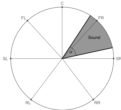
Figure 13.31. The focus angle \alpha defines the projection of an extended sound source on the speaker circle.
