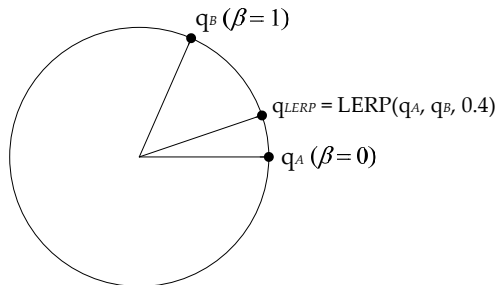
Figure 4.23. Linear interpolation (LERP) between two quaternions q_A and q_B .
