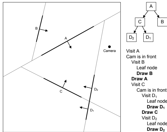
Figure 10.51. An example of back-to-front traversal of the triangles in a BSP tree. The triangles are shown edge-on in two dimensions for simplicity, but in a real BSP tree the triangles and dividing planes would be arbitrarily oriented in space.
