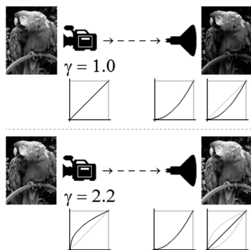
Figure 10.66. The effect of a CRT's gamma response on image quality and how the effect can be corrected for. Image courtesy of www.wikipedia.org .
