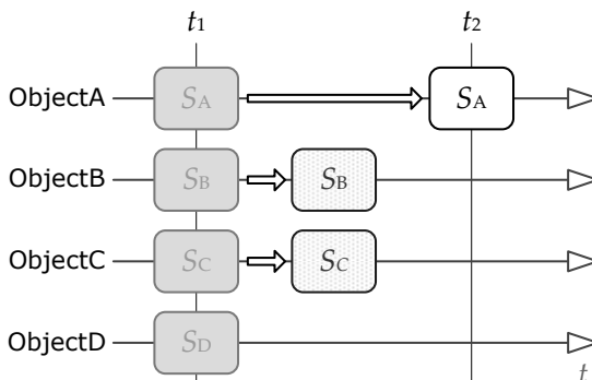
Figure 15.16. In practice, the states of the game objects are updated one by one. This means that at some arbitrary moment during the update loop, some objects will think the current time is t_2 while others think it is still t_1 . Some objects may be only partially updated, so their states will be internally inconsistent. In effect, the state of such an object lies at a point between t_1 and t_2 .
