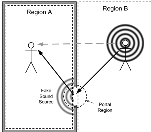
Figure 13.36. The portal-based audio propagation model used in The Last of Us by Naughty Dog, Inc.
