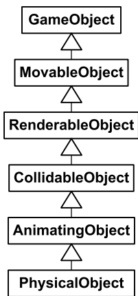
Figure 15.7. A hypothetical game object class hierarchy using only inheritance to associate the classes.
