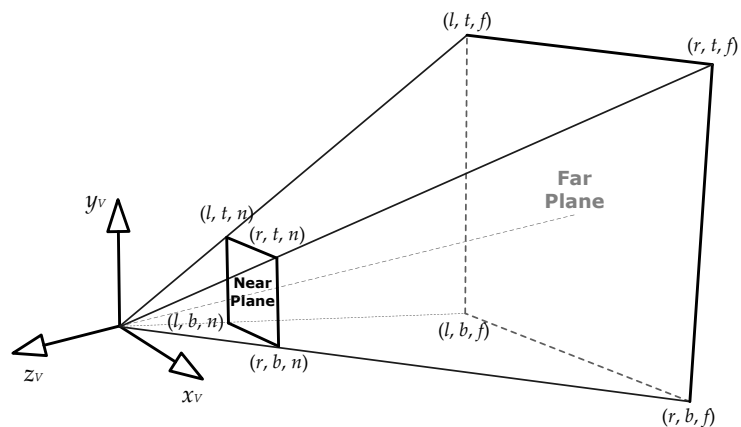
Figure 10.33. A perspective view volume (frustum).
