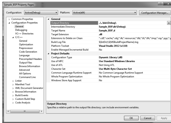
Figure 2.10. Visual Studio project property pages—General page.
