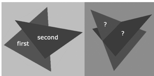
Figure 10.38. The painter's algorithm renders triangles in a back-to-front order to produce proper triangle occlusion. However, the algorithm breaks down when triangles intersect one another.
