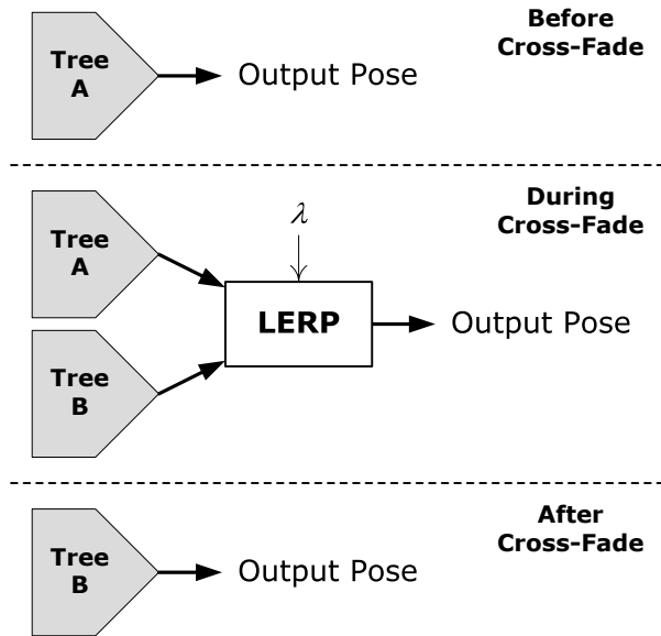
Figure 11.55. A cross-fade between two arbitrary blend trees A and B.
