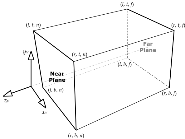
Figure 10.34. An orthographic view volume.
