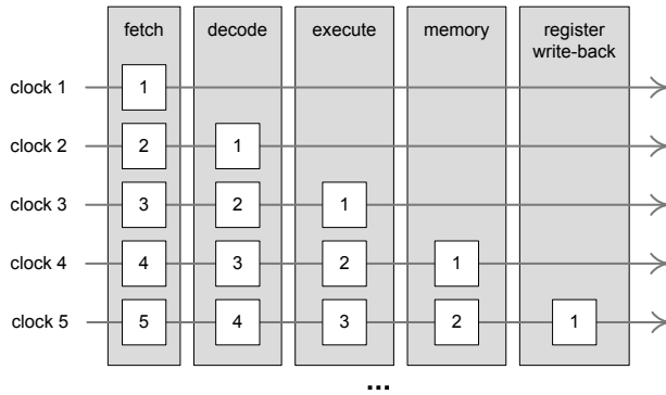
Figure 3.22. The flow of instructions through a pipelined CPU.
