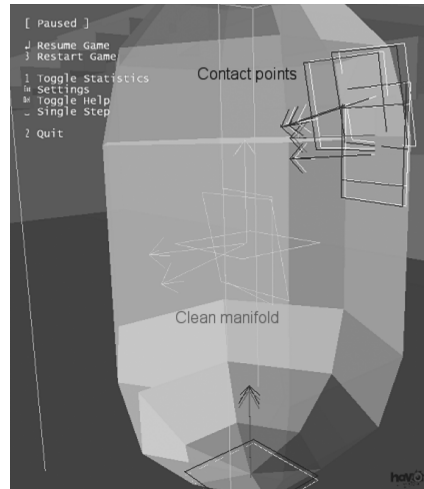
Figure 12.36. Havok’s character controller models a character as a capsule-shaped phantom. The phantom maintains a noise-reduced collision manifold (a collection of contact planes) that can be used by the game to make movement decisions.
