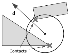
Figure 12.19. A cast sphere that starts in penetration will be unable to move, and possibly many contact points will lie inside the cast shape in general.
