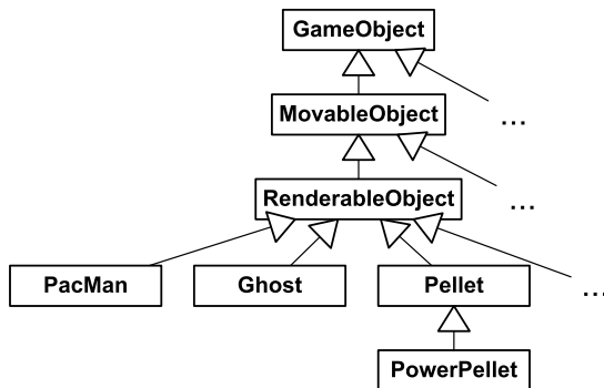
Figure 15.2. A hypothetical class hierarchy for the game Pac-Man .
