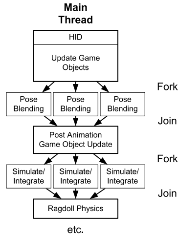
Figure 7.8. Fork and join used to parallelize selected CPU-intensive parts of the game loop.
