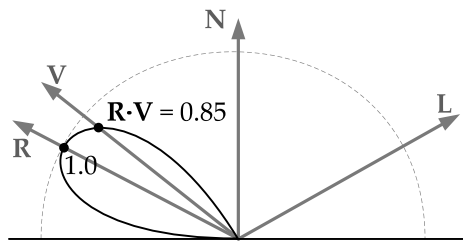
Figure 10.26. The specular term of the Phong reflection model is at its maximum when the viewing angle \mathbf{V} coincides with the reflected light direction \mathbf{R} and drops off quickly as \mathbf{V} diverges from \mathbf{R} .
