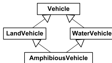
Figure 15.5. A diamond-shaped class hierarchy for amphibious vehicles.
