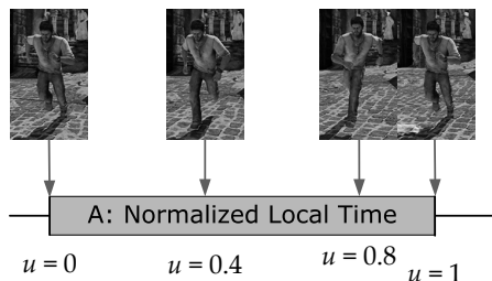
Figure 11.13. An animation clip, showing normalized time units. Images courtesy of Naughty Dog, Inc., © 2014/™ SCEA.
