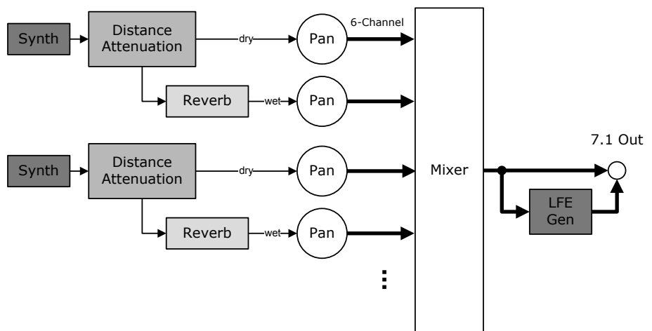
Figure 13.39. The audio processing graph (pipeline).
