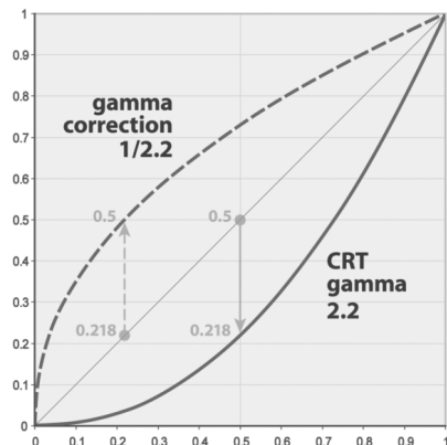
Figure 10.67. Gamma encoding and decoding curves. Image courtesy of www.wikipedia.org .
