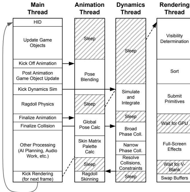
Figure 7.9. One thread per major engine subsystem.
