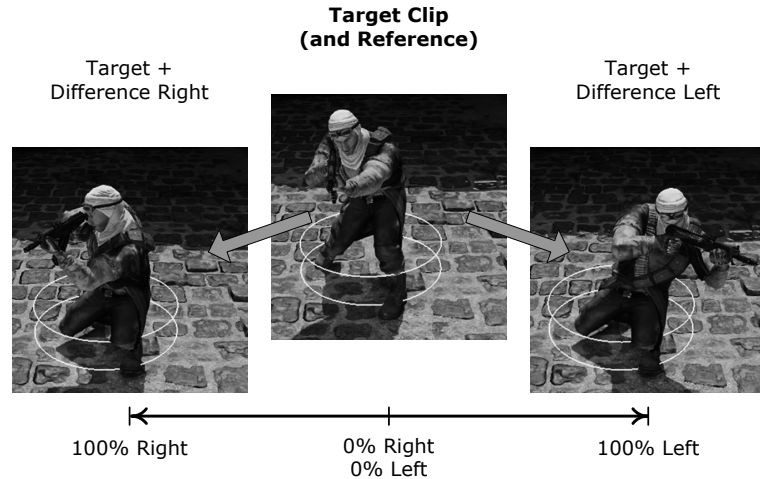
Figure 11.40. Additive blending can be used to aim a weapon. Screenshots courtesy of Naughty Dog, Inc., © 2014/™ SCEA.
