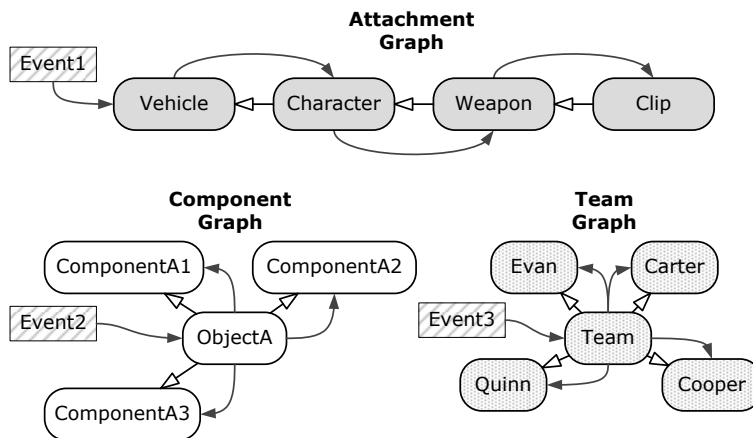
Figure 15.17. Game objects are interrelated in various ways, and we can draw graphs depicting these relationships. Any such graph might serve as a distribution channel for events.
