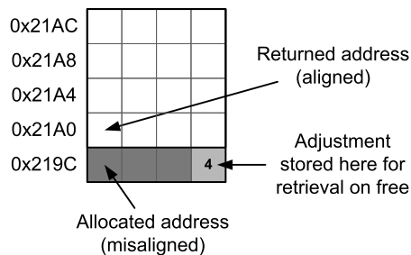
Figure 5.3. Aligned memory allocation with a 16-byte alignment requirement. The difference between the allocated memory address and the adjusted (aligned) address is stored in the byte immediately preceding the adjusted address, so that it may be retrieved during free.
