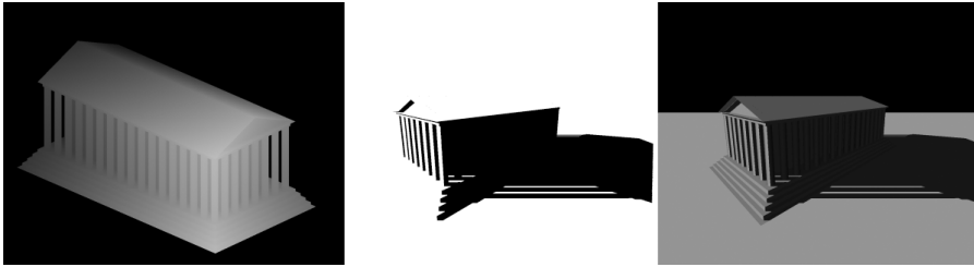
Figure 10.57. The far left image is a shadow map—the contents of the z -buffer as rendered from the point of view of a particular light source. The pixels of the center image are black where the light-space depth test failed (fragment in shadow) and white where it succeeded (fragment not in shadow). The far right image shows the final scene rendered with shadows.
