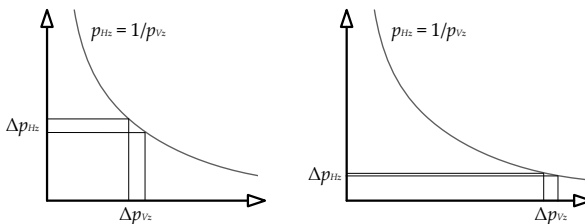
Figure 10.39. A plot of the function 1/p_{V_z} , showing how most of the precision lies close to the camera.
