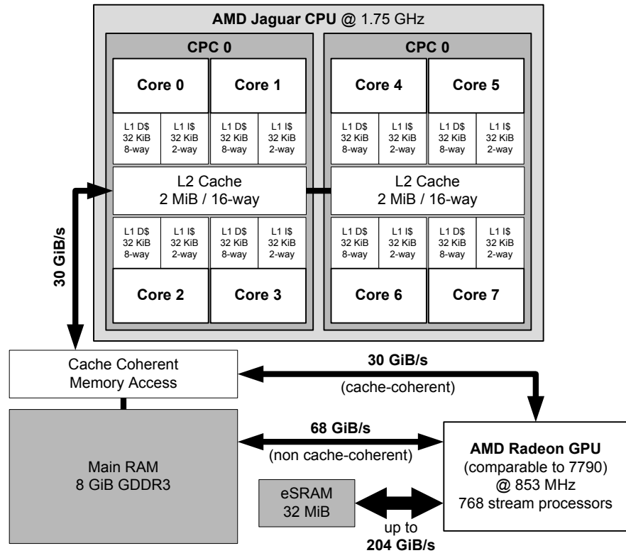
Figure 7.7. Simplified view of the Xbox One's architecture.
