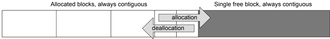
Figure 5.5. A stack allocator is free from fragmentation problems.
