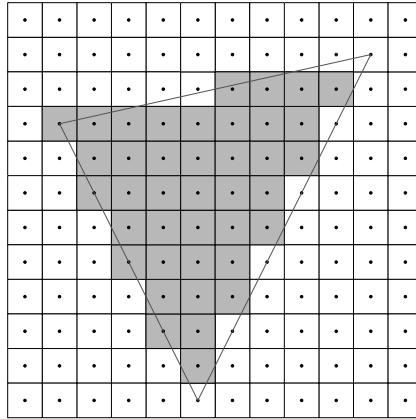
Figure 10.46. Rasterizing a triangle without antialiasing.
