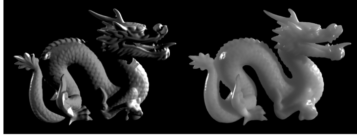
Figure 10.61. On the left, a dragon rendered without subsurface scattering (i.e., using a BRDF lighting model). On the right, the same dragon rendered with subsurface scattering (i.e., using a BSSRDF model). Images rendered by Rui Wang at the University of Virginia.
