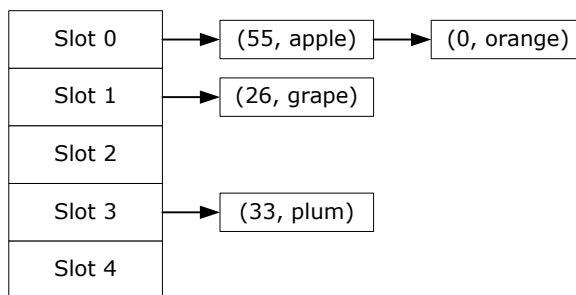
Figure 5.10. An open hash table.
