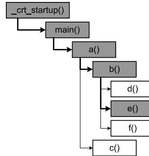
Figure 9.13. Call stack resulting from setting a breakpoint in function e() .
