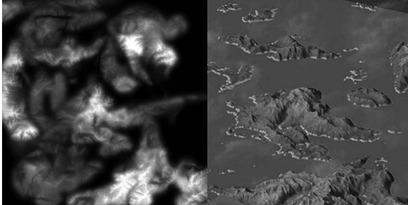
Figure 10.65. A grayscale height field bitmap (left) can be used to control the vertical positions of the vertices in a terrain grid mesh (right). In this example, a water plane intersects the terrain mesh to create islands.
