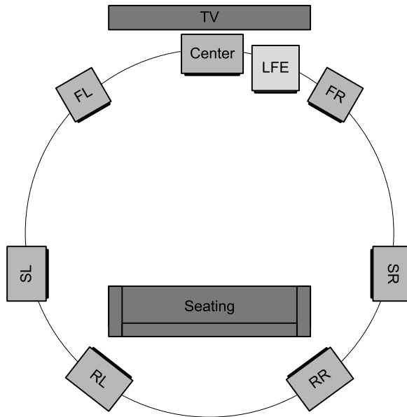
Figure 13.24. Speaker arrangement for a 7.1 surround sound home theater system.
