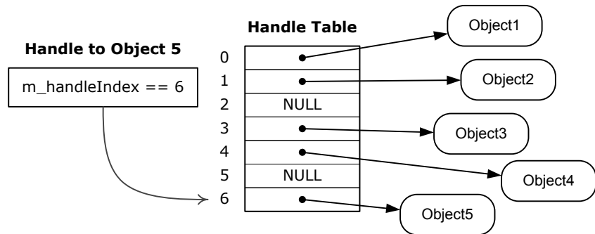
Figure 15.13. A handle table contains raw object pointers. A handle is simply an index into this table.
