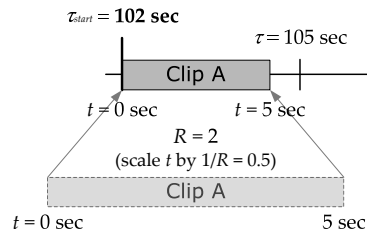
Figure 11.16. Playing an animation at twice the speed corresponds to scaling its local timeline by a factor of 1/2 .
