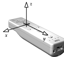
Figure 8.9. Accelerometer axes for the Wiimote.
