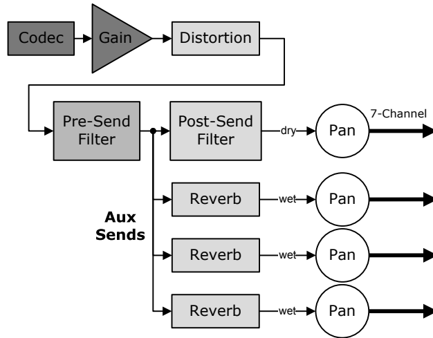
Figure 13.40. The pipeline through which an individual 3D voice passes on its way through the audio graph.
