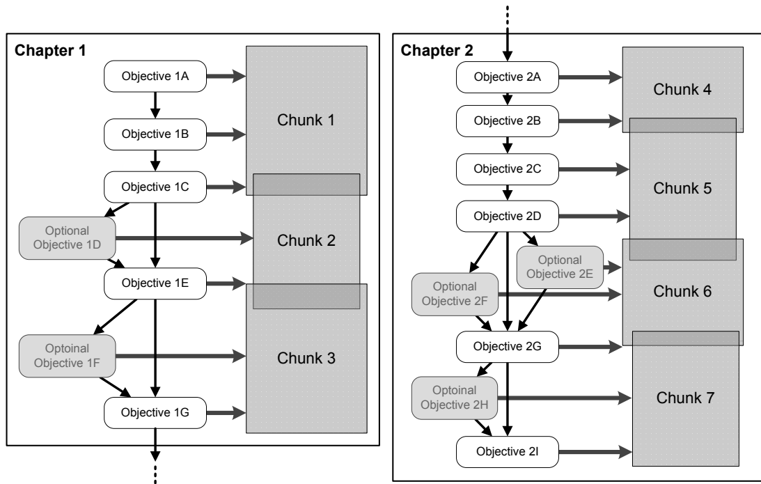
Figure 14.3. Gameplay objectives are typically arranged in a sequence, tree or graph, and each one maps to one or more game world chunks.
