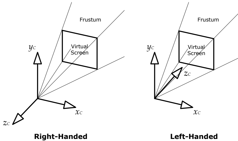
Figure 10.31. Left- and right-handed camera-space axes.
