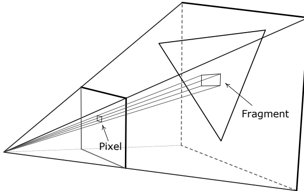
Figure 10.37. A fragment is a small region of a triangle corresponding to a pixel on the screen. It passes through the rendering pipeline and is either discarded or its color is written into the frame buffer.
