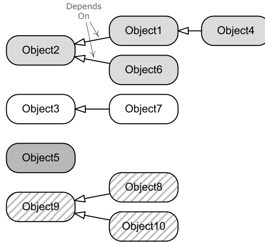
Figure 15.14. Inter-object update order dependencies can be viewed as a forest of dependency trees.
