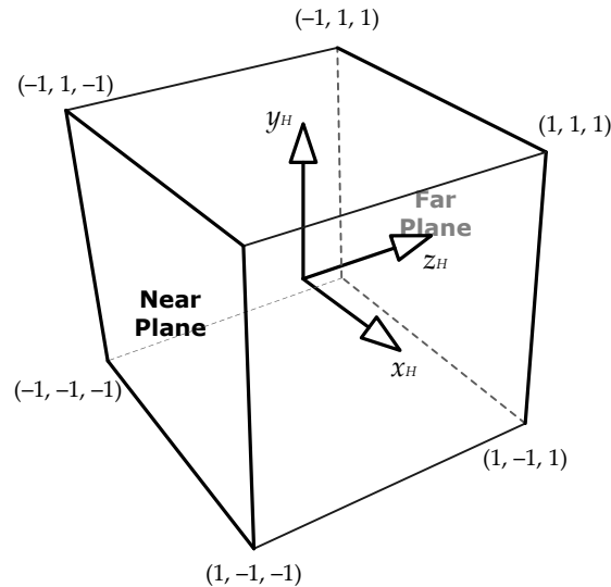
Figure 10.35. The canonical view volume in homogeneous clip space.
