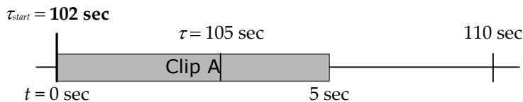
Figure 7.1. Playing an animation clip can be visualized as mapping its local timeline onto the global game timeline.
