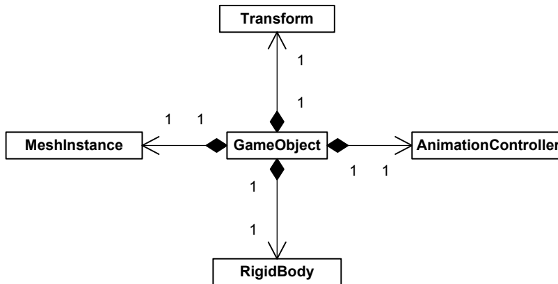
Figure 15.8. Our hypothetical game object class hierarchy, refactored to favor class composition over inheritance.
