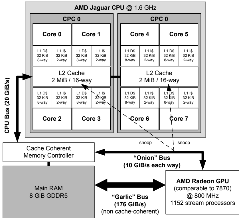
Figure 7.6. Simplified view of the PS4's architecture.
