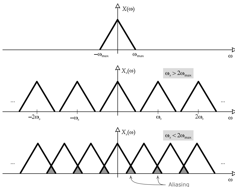
Figure 13.26. The frequency spectrum of a band-limited signal is zero everywhere except within a limited frequency band (top). If the sampling frequency exceeds the Nyquist frequency, the spectrum copies do not overlap and the original signal can be recovered exactly (middle). If the sampling frequency is too low, the spectrum copies overlap and aliasing results (bottom).
