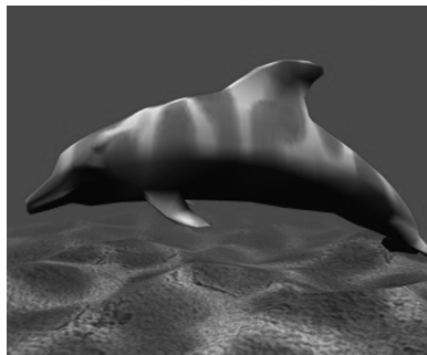
Figure 10.60. Water caustics produced by projecting an animated texture onto the affected surfaces.
