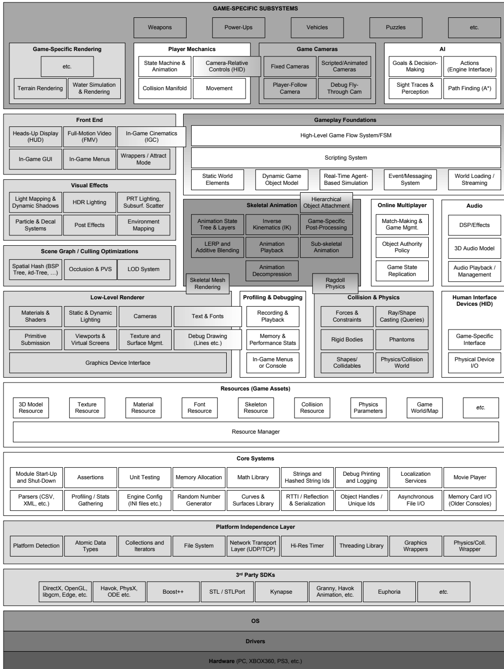
Figure I.15. Runtime game engine architecture.
