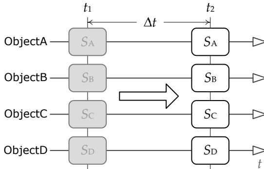
Figure 15.15. In theory, the states of all game objects are updated instantaneously and in parallel during each iteration of the game loop.
