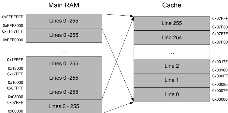
Figure 3.19. Direct mapping between main memory addresses and cache lines.
