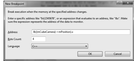
Figure 2.16. Defining a data breakpoint.
