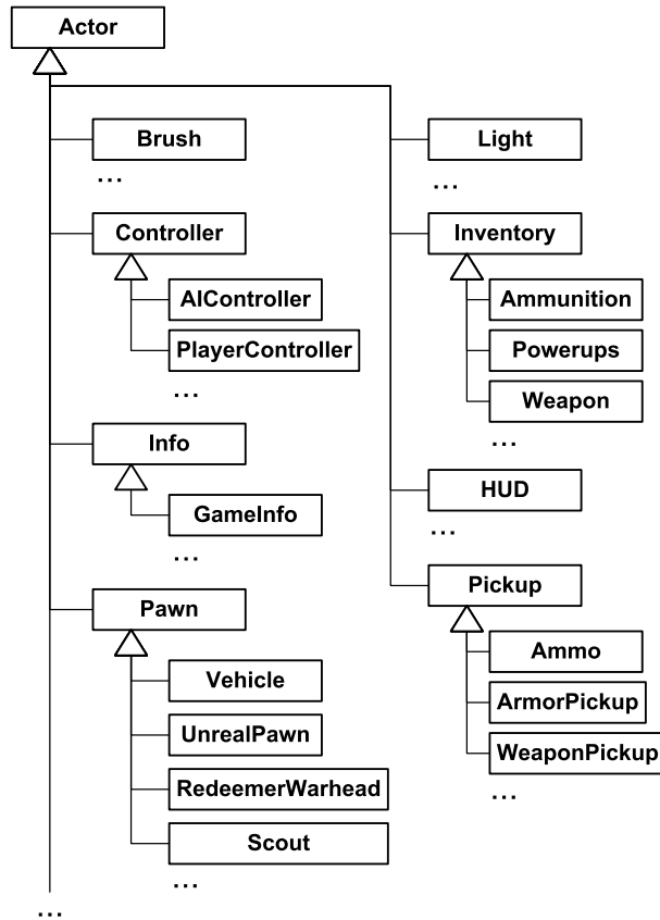
Figure 15.3. An excerpt from the game object class hierarchy in the Unreal engine.
