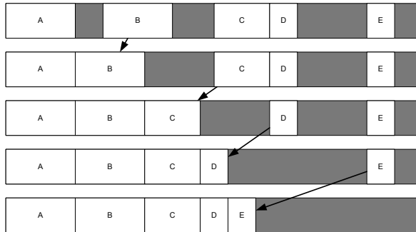
Figure 5.7. Defragmentation by shifting allocated blocks to lower addresses.
