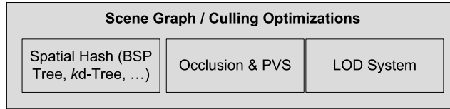
Figure 1.24. A typical scene graph/spatial subdivision layer, for culling optimization.
