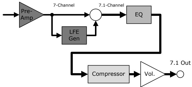
Figure 13.41. A typical master output bus.
