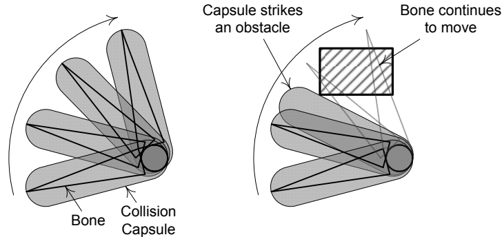
Figure 12.34. With a powered rag doll constraint, and in the absence of any additional forces or torques, a rigid body representing the lower arm can be made to exactly track the movements of an animated elbow joint (left). If an obstacle blocks the motion of the body, it will diverge from that of the animated elbow joint in a realistic way (right).
