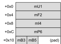
Figure 3.15. More efficient packing by grouping small members together.
