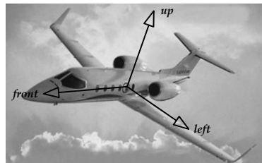
Figure 4.18. One possible choice of the model-space front, left and up axis basis vectors for an airplane.
