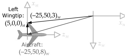
Figure 4.19. A Lear jet whose left wingtip is at (5, 0, 0) in model space. If the jet is rotated by 90 degrees about the world-space y -axis, and its model-space origin translated to (-25, 50, 8) in world space, then its left wingtip would end up at (-25, 50, 3) when expressed in world-space coordinates.
