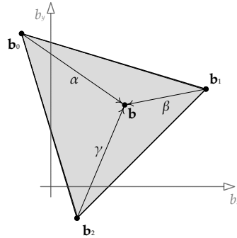
Figure 11.36. Various barycentric coordinates within a triangle.
