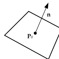
Figure 4.29. A plane in point-normal form.
