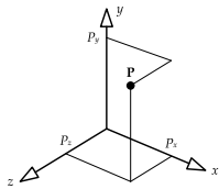
Figure 4.1. A point represented in Cartesian coordinates.
