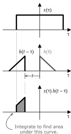
Figure 13.15. Visualization of the convolution operation in continuous time.
