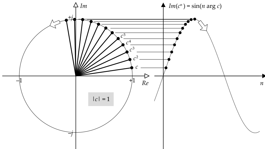
Figure 13.19. Multiplying a complex number by itself repeatedly traces out a circular path in the Argand plane, producing a sinusoid when projected onto any axis through the origin.
