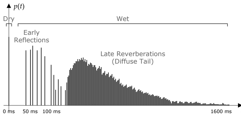
Figure 13.6. Direct sound waves, early reflections and late reverberations.
