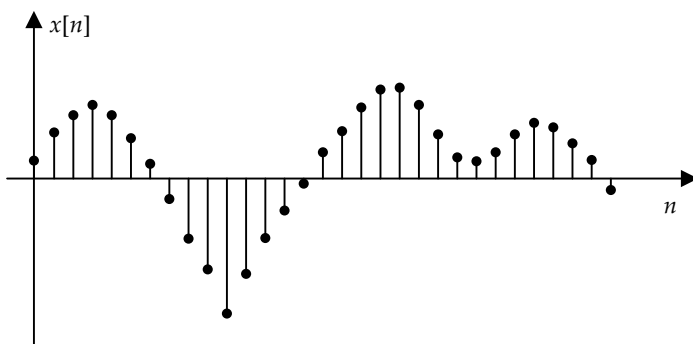
Figure 13.7. The value of a discrete-time signal x[n] is defined only for integer values of n .
