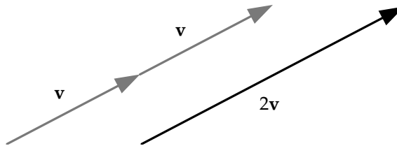
Figure 4.5. Multiplication of a vector by the scalar 2.
