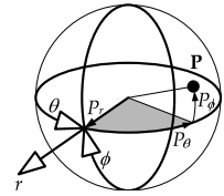
Figure 4.3. A point represented in spherical coordinates.
