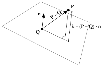
Figure 4.12. The dot product can be used to find the height of a point above or below a plane.
