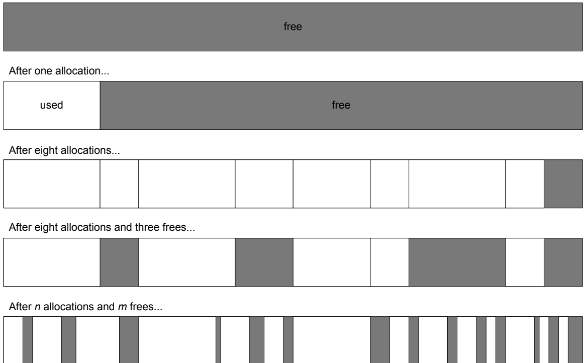
Figure 5.4. Memory fragmentation.
