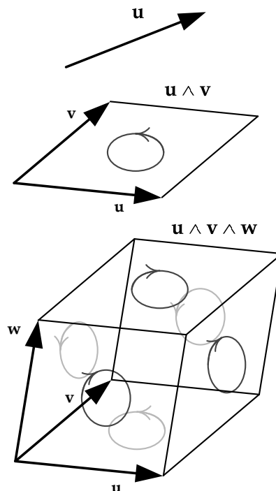
Figure 4.15. In the exterior algebra (Grassman algebra), a single wedge product yields a pseudovector or bivector, and two wedge products yields a pseudoscalar or trivector.
