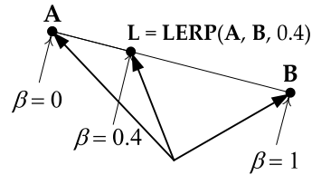
Figure 4.16. Linear interpolation (LERP) between points A and B , with \beta = 0.4 .
