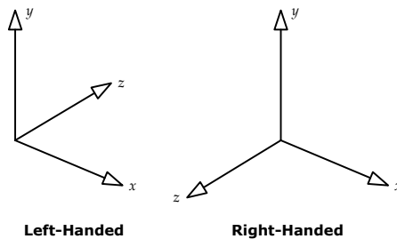
Figure 4.4. Left- and right-handed Cartesian coordinate systems.
