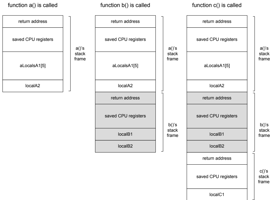
Figure 3.10. Stack frames.
