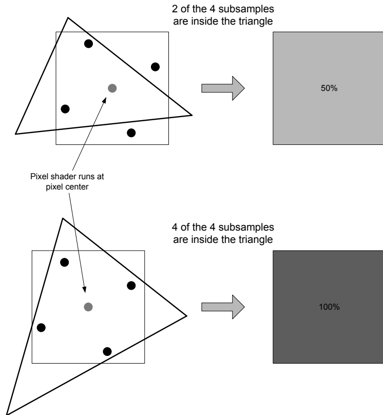
Figure 10.47. Multisampled antialiasing (MSAA).
