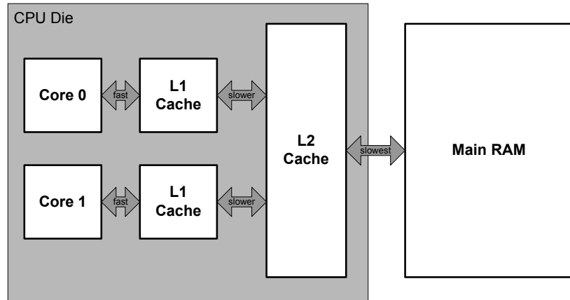
Figure 3.21. Level 1 and level 2 caches.
