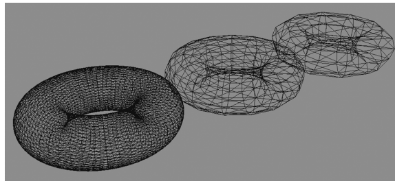
Figure 10.4. A chain of LOD meshes, each with a fixed level of tessellation, can be used to approximate uniform triangle-to-pixel density. The leftmost torus is constructed from 5000 triangles, the center torus from 450 triangles and the rightmost torus from 200 triangles.
