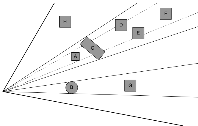
Figure 10.49. As a result of the antiportals corresponding to objects A, B and C, objects D, E, F and G are culled. Therefore, only A, B, C and H are visible.
