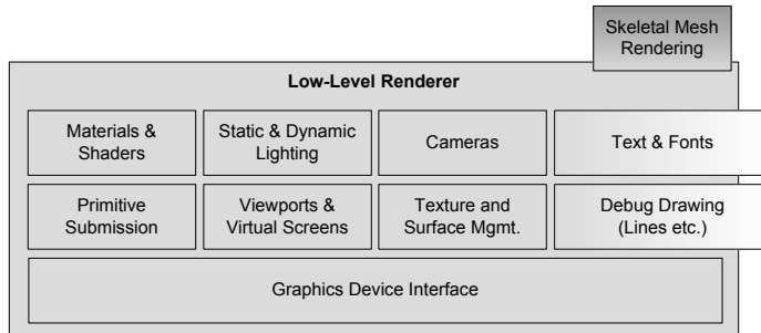
Figure 1.23. Low-level rendering engine.
