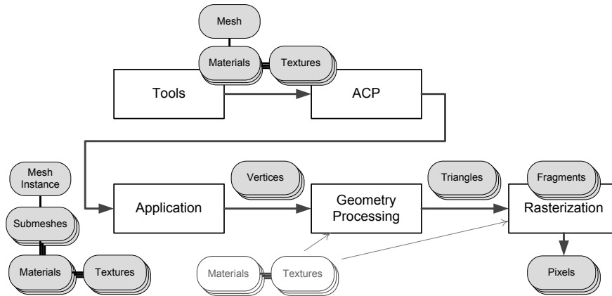
Figure 10.41. The format of geometric data changes radically as it passes through the various stages of the rendering pipeline.
