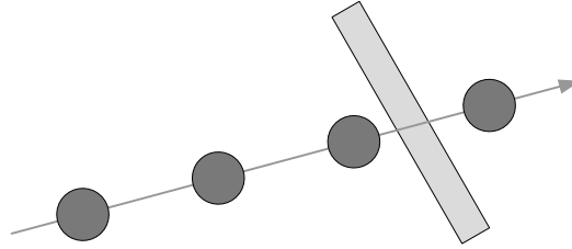
Figure 12.16. A small, fast-moving object can leave gaps in its motion path between consecutive snapshots of the collision world, meaning that collisions might be missed entirely.
