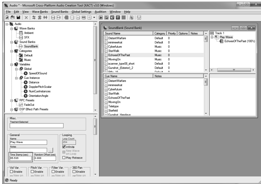
Figure 13.42. Microsoft's XACT audio authoring tool for Windows and Xbox platforms.
