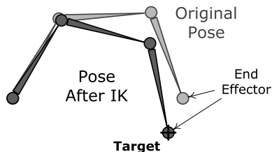
Figure 11.41. Inverse kinematics attempts to bring an end effector joint into a target global pose by minimizing the error between them.
