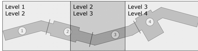
Figure 15.12. A game world divided into chunks. Level load regions, each with a requested chunk list, are arranged in such a way as to guarantee that the player never sees a chunk pop in or out of view.
