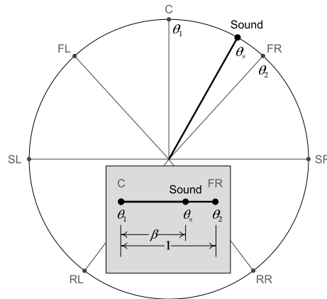
Figure 13.30. Treating the sound as a point source, the pan blend percentage \beta is calculated between the two speakers immediately adjacent to the source.
