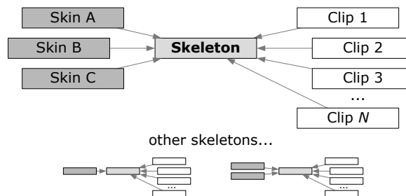
Figure II.46. Many animation clips and one or more meshes target a single skeleton.
