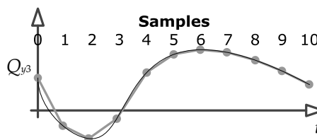
Figure 11.22. Many game engines use a piecewise linear approximation when interpolating channel functions.
