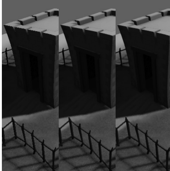
Figure 10.45. No antialiasing (left), 4× MSAA (center) and Nvidia's FXAA, preset 3 (right). Image from Nvidia's FXAA white paper by Timothy Lottes ( http://bit.ly/1mlzCTv ). (See Color Plate XVIII.)
