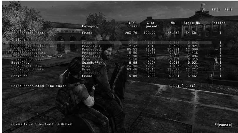
Figure 9.10. The Naughty Dog engine provides a profile hierarchy display that allows the user to drill down into particular function calls to inspect their costs.
