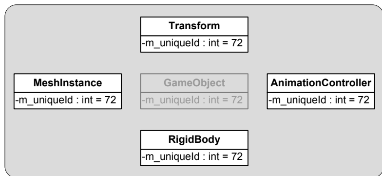
Figure 15.10. In a pure component model, a logical game object is comprised of many components, but the components are linked together only indirectly, by sharing a unique id.
