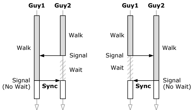
Figure 15.20. Two examples showing how a simple pattern of raising one signal and then waiting on another can be used to synchronize a pair of script threads.
