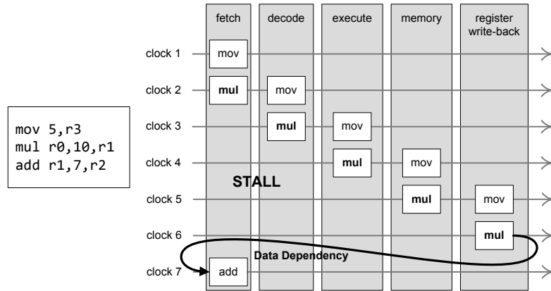
Figure 3.23. A data dependency between instructions causes a pipeline stall.
