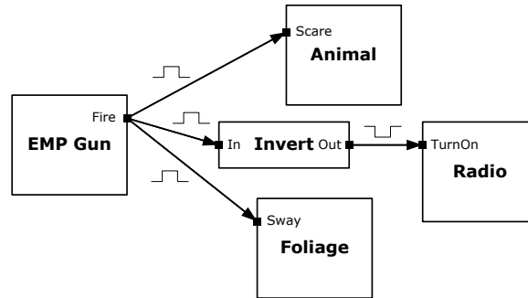
Figure 15.18. The EMP gun produces a 1 at its “Fire” output when fired. This can be connected to any input port that expects a Boolean value, in order to trigger the behavior associated with that input.
