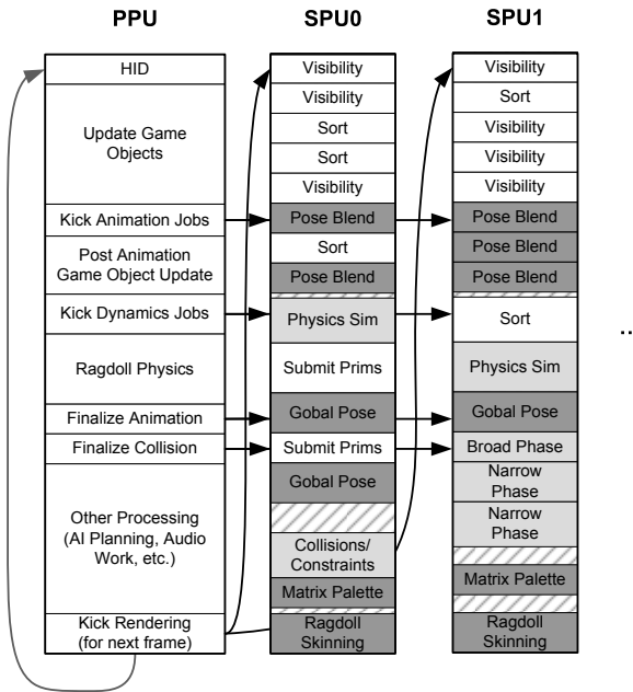
Figure 7.10. In a job model, work is broken down into fine-grained chunks that can be picked up by any available processor. This can help maximize processor utilization while providing the main game loop with improved flexibility.
