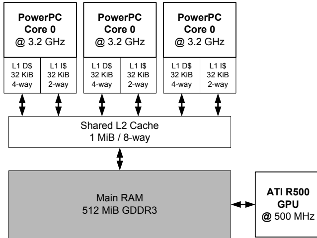
Figure 7.4. A simplified view of the Xbox 360 hardware architecture.
