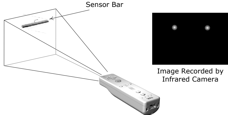
Figure 8.10. The Wii sensor bar houses two infrared LEDs, which produce two bright spots on the image recorded by the Wiimote's IR camera.
