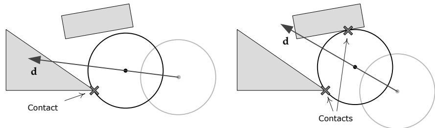
Figure 12.20. If the starting location of a cast shape is not interpenetrating anything, then the shape will move a nonzero distance along its line segment, and its contacts (if any) will always be on its surface.
