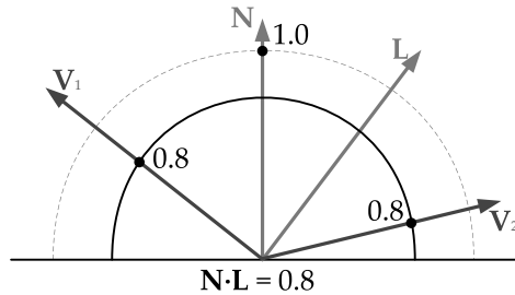
Figure 10.25. The diffuse term of the Phong reflection model is dependent upon \mathbf{N} \cdot \mathbf{L} but is independent of the viewing angle \mathbf{V} .
