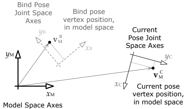
Figure 11.24. Bind pose and current pose of a simple, one-joint skeleton and a single vertex bound to that joint.
