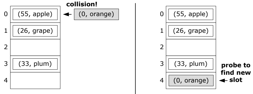
Figure 5.II. A closed hash table.
