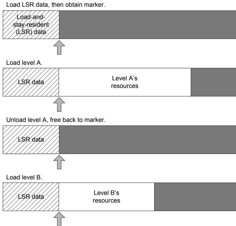
Figure 15.II. A stack-based memory allocator is extremely well-suited to a one-level-at-a-time world loading system.
