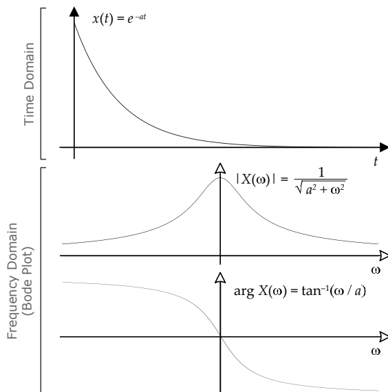
Figure 13.20. The Fourier transform yields a complex-valued frequency domain signal. A Bode plot is used to visualize this complex-valued signal in terms of its magnitude and its phase (or argument).
