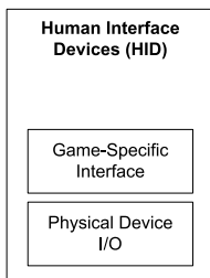
Figure 1.30. The player input/output system, also known as the human interface device (HID) layer.
