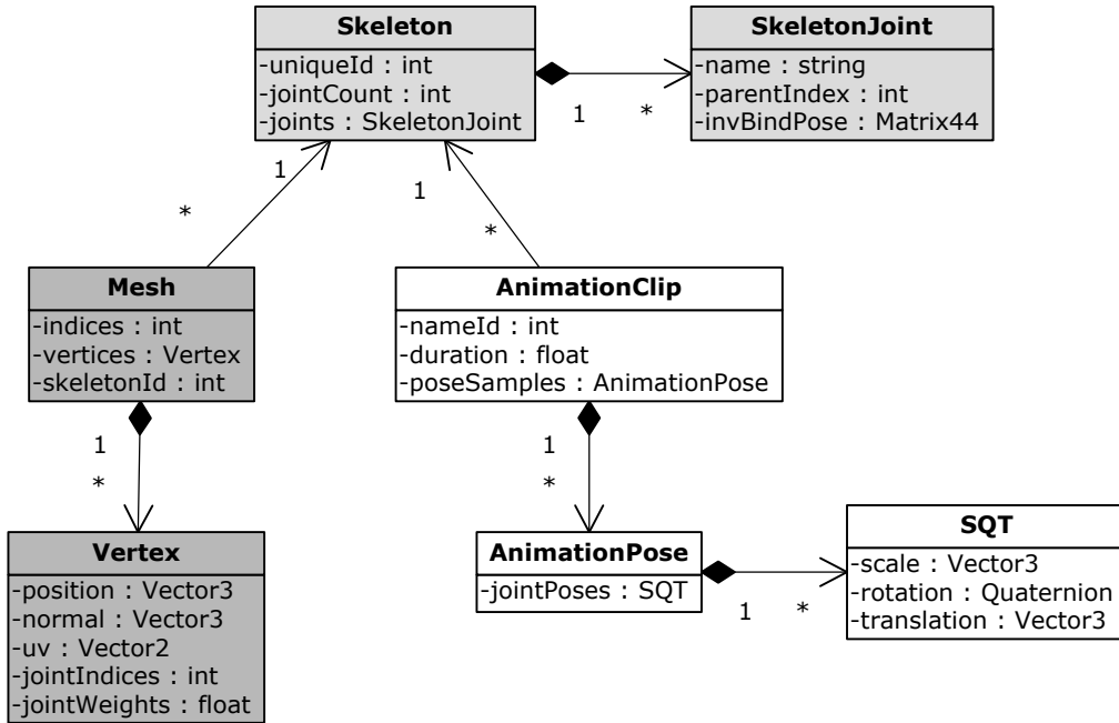
Figure II.45. UML diagram of shared animation resources.
