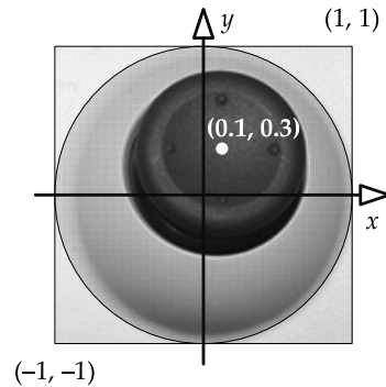
Figure 8.8. Two analog inputs can be used to represent the x and y deflection of a joystick.
