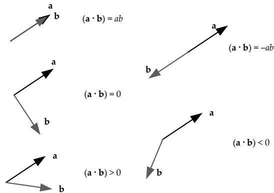
Figure 4.11. Some common dot product tests.
