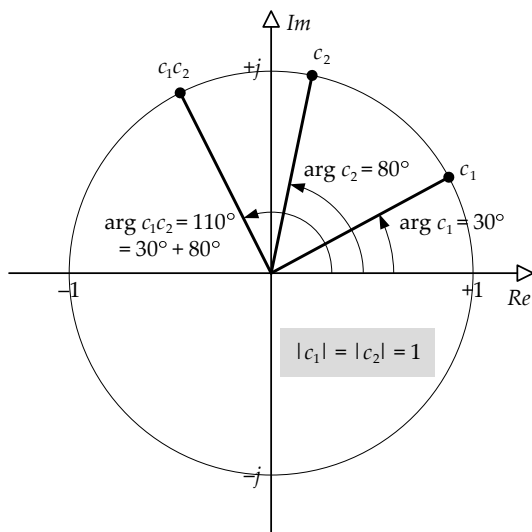
Figure 13.17. Multiplying two complex numbers together that both have magnitudes of 1 produces a pure rotation in the complex plane.
