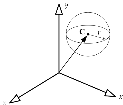
Figure 4.28. Point-radius representation of a sphere.
