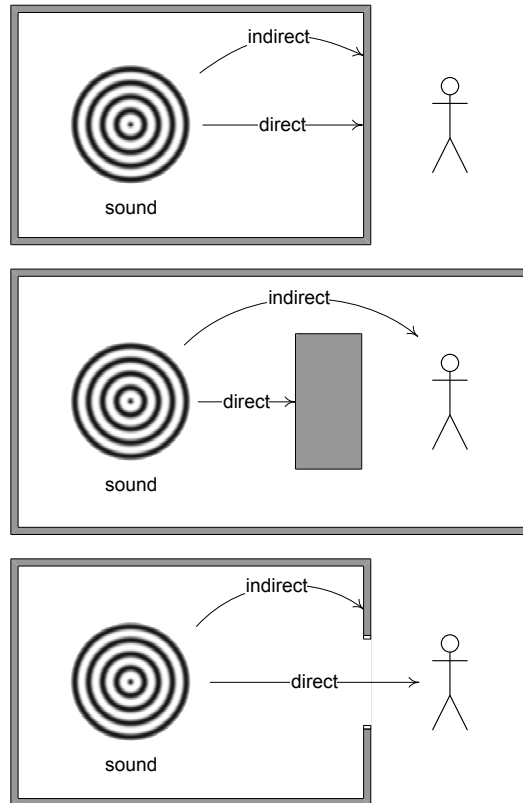
Figure 13.33. From top to bottom: occlusion, obstruction and exclusion.
