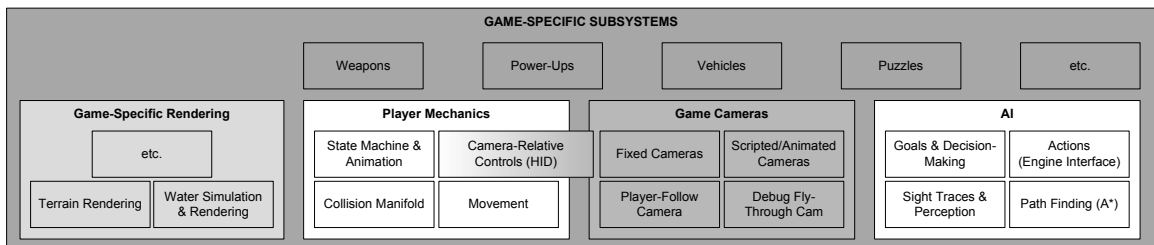
Figure 1.34. Game-specific subsystems.
