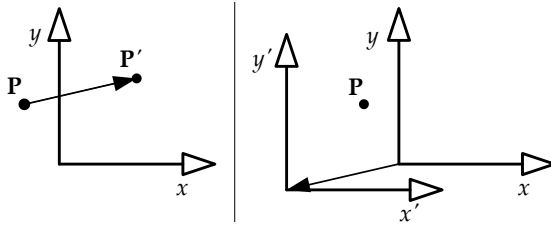
Figure 4.22. Two ways to interpret a transformation matrix. On the left, the point moves against a fixed set of axes. On the right, the axes move in the opposite direction while the point remains fixed.
