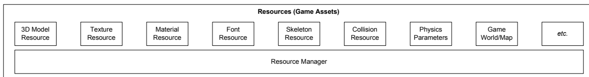
Figure 1.22. Resource manager.
