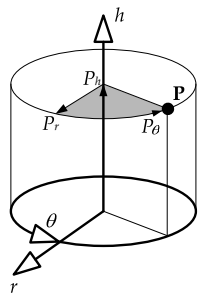
Figure 4.2. A point represented in cylindrical coordinates.
