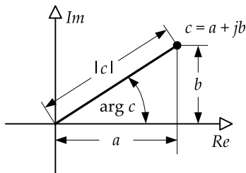
Figure 13.16. The magnitude |c| = \sqrt{a^2 + b^2} of a complex number is its length in the complex plane, and its argument \arg c = \tan^{-1}(b/a) is the angle it makes with the \Re axis.
