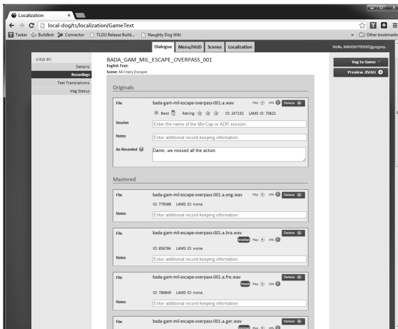
Figure 5.16. Detailed asset view showing recorded translations for the speech asset BADA_GAM_MIL_ESCAPE_OVERPASS_001 ("We missed all the action").
