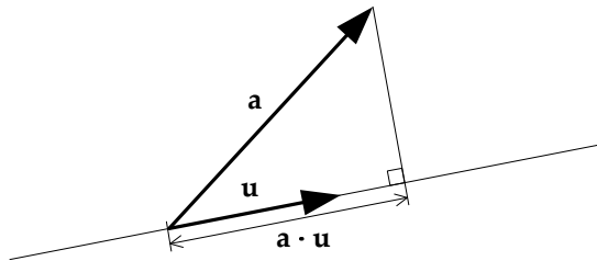
Figure 4.10. Vector projection using the dot product.
