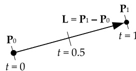
Figure 4.27. Parametric equation of a line segment, with normalized parameter t .
