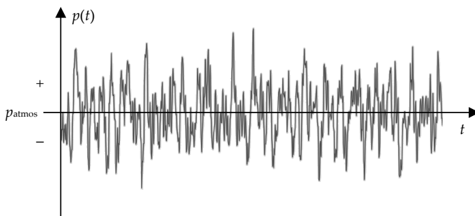
Figure 13.1. A signal p(t) can be used to model the time-varying acoustic pressure of a sound.
