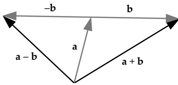
Figure 4.6. Vector addition and subtraction.
