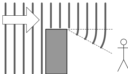
Figure 13.34. Diffraction causes the dry component of a sound to be clearly audible even when the direct path is blocked.
