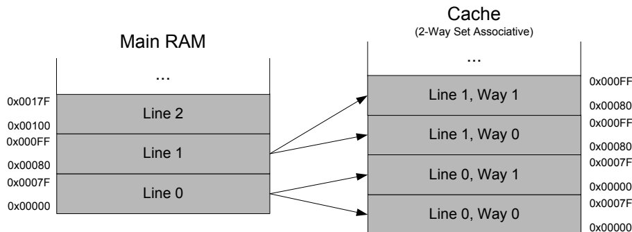
Figure 3.20. A 2-way set associative cache.
