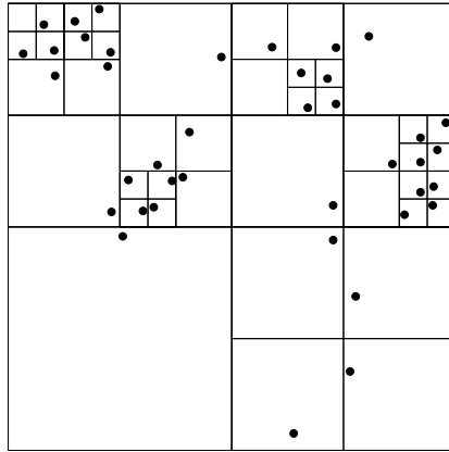
Figure 10.50. A top-down view of a space divided recursively into quadrants for storage in a quadtree, based on the criterion of one point per region.
