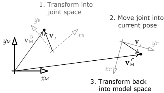
Figure 11.25. By transforming a vertex's position into joint space, it can be made to "track" the joint's movements.
