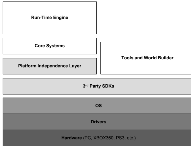
Figure 1.36. Stand-alone tools architecture.
