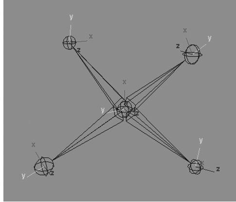
Figure 11.7. Every joint in a skeletal hierarchy defines a set of local coordinate space axes, known as joint space.
