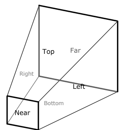
Figure 4.30. A frustum.
