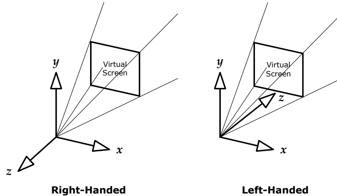
Figure 4.20. Left- and right-handed examples of view space, also known as camera space.
