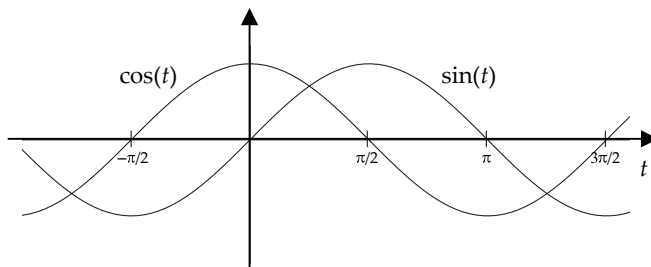
Figure 13.3. The sine and cosine functions are just phase-shifted versions of one another.
