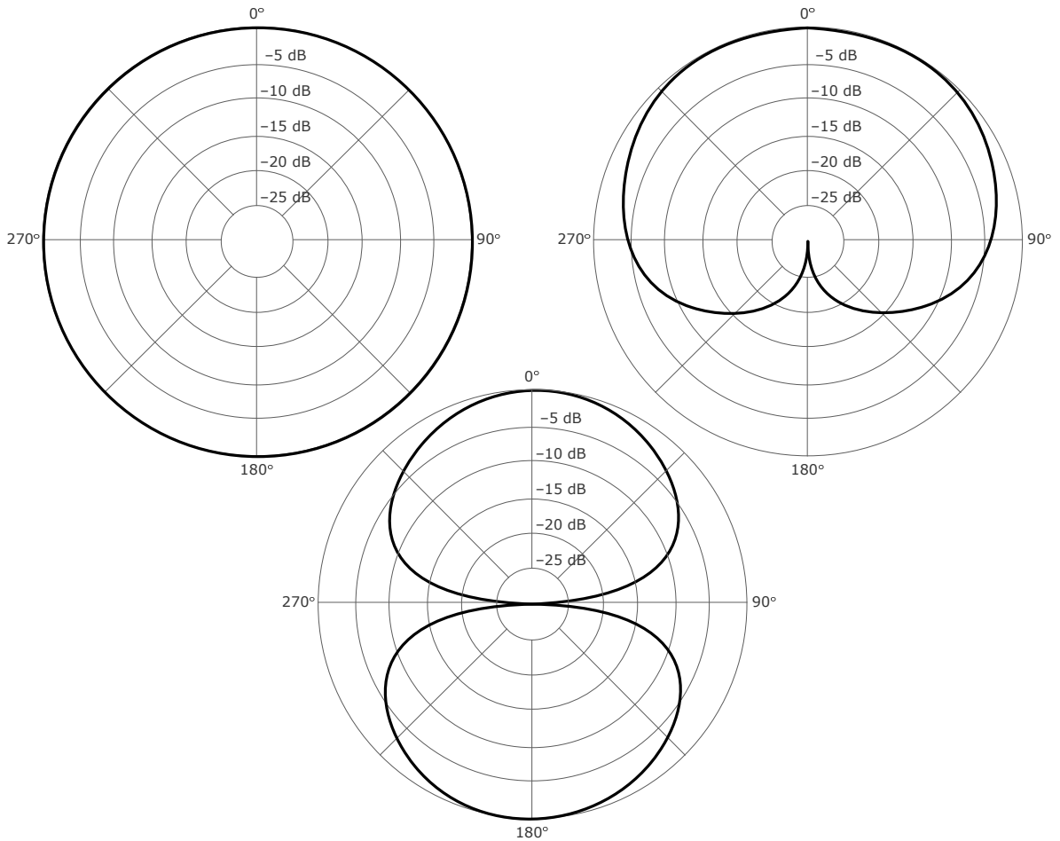
Figure 13.23. Three typical microphone polar patterns, clockwise from upper left: omnidirectional, cardioid and bidirectional.
