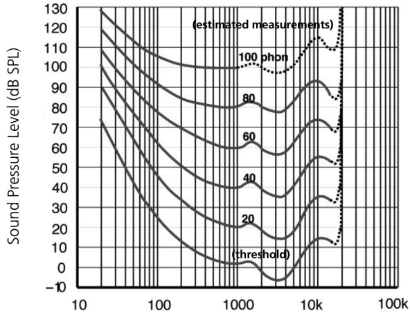
Figure 13.4. The human ear is most sensitive in the frequency range between 2 and 5 kHz. As the frequency decreases or increases beyond this range, more and more acoustic pressure is required to produce the same perception of “loudness.”
